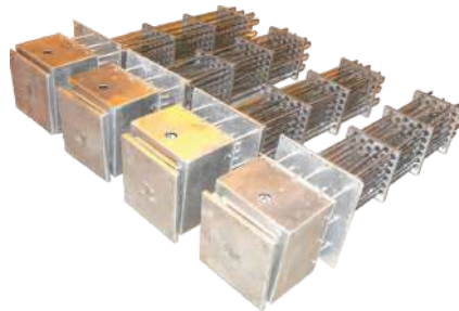
Purge Air Heater for Thermal Power Plant
