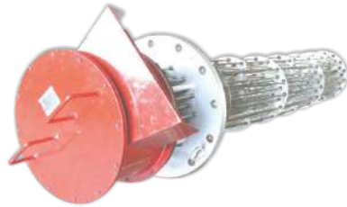
Heater For Spray Drying Applications, Rating From 6kw To 200kw
